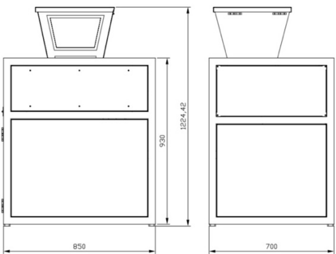
Fig. 4: L×W×H (mm) Fits through office doors and elevators
